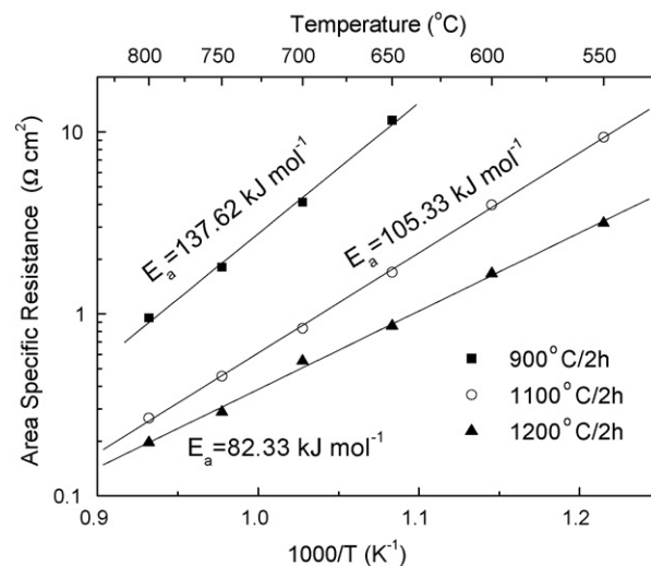
Fig. 2. Area-specific resistance (ASR) results for the symmetrical cells of PBSC–BZCY sintered in air for 2 h at 900, 1100 and 1200 °C, respectively.
