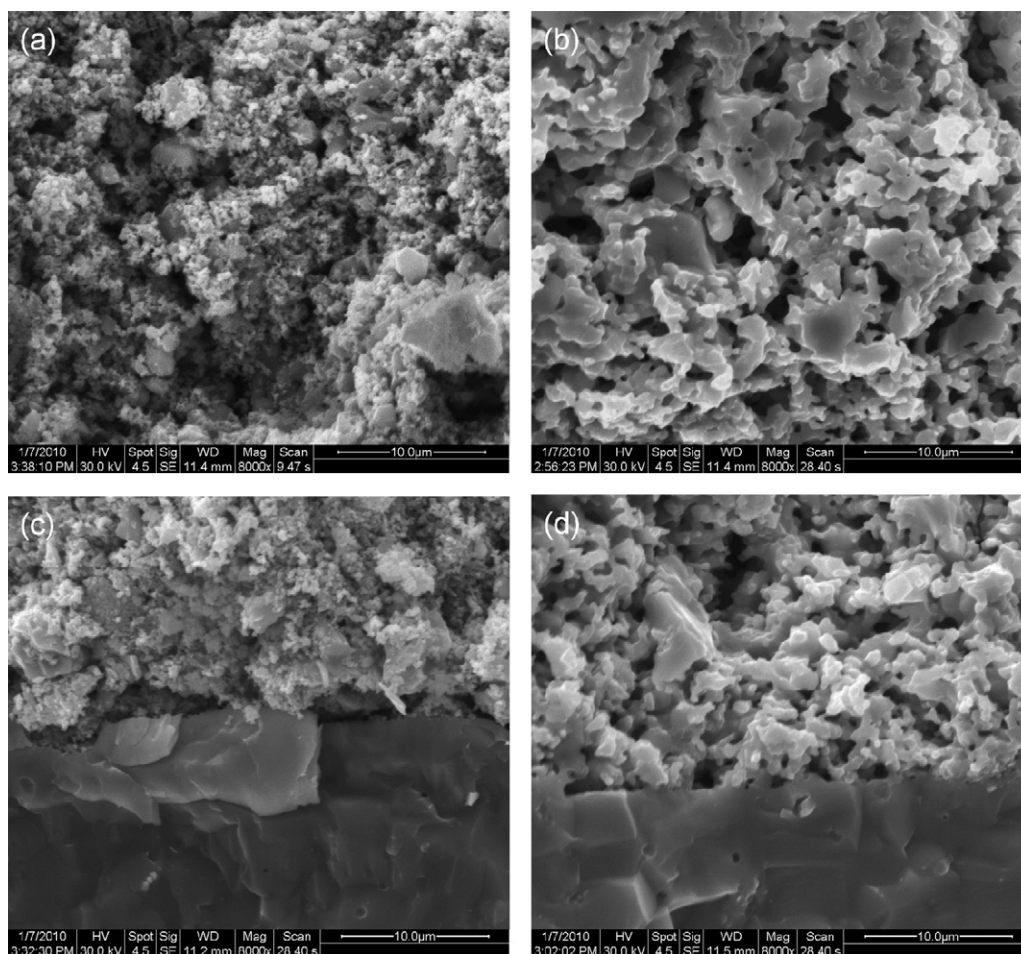
Fig. 3. Cross-section images of the post-examined symmetrical cathodes. PBSC–BZCY bulk for cathode sintered at 900 °C (a) and 1200 °C (b) for 2 h; cathode (PBSC–BZCY)/electrolyte (BZCY) interface sintered at 900 °C (c) and 1200 °C (d) for 2 h.
