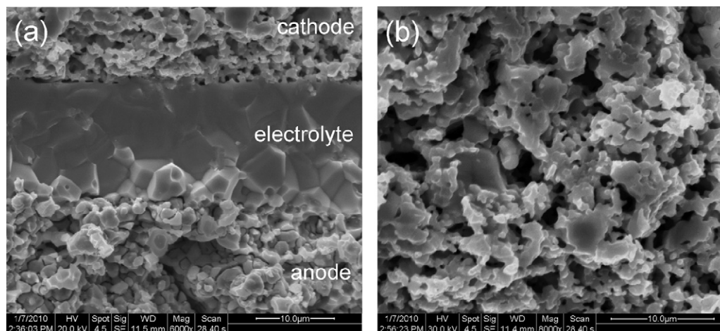
Fig. 7. Cross-section images of the post-examined single cell: (a) the cell with a 15 \mu\text{m} thick BZCY membrane and (b) the PBSC–BZCY composite cathode.
