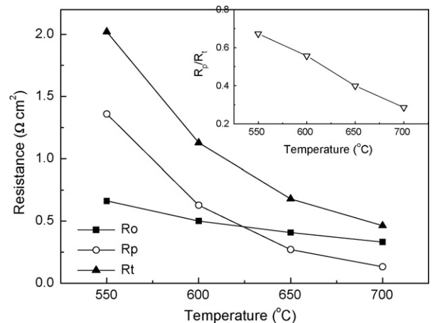
Fig. 6. The interfacial polarization resistances ( R_p ), ohmic resistances ( R_o ), total resistances ( R_t ), and the ratio of interfacial polarization resistance to total resistance ( R_p/R_t ) obtained from the impedance spectra at different temperatures of the cell.
