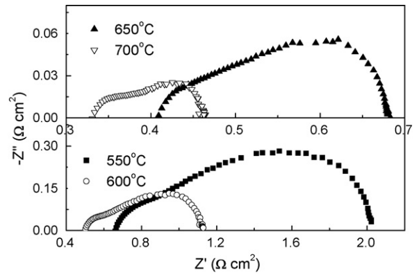
Fig. 5. Impedance spectra of the cell measured under open-circuit conditions at different temperatures.
