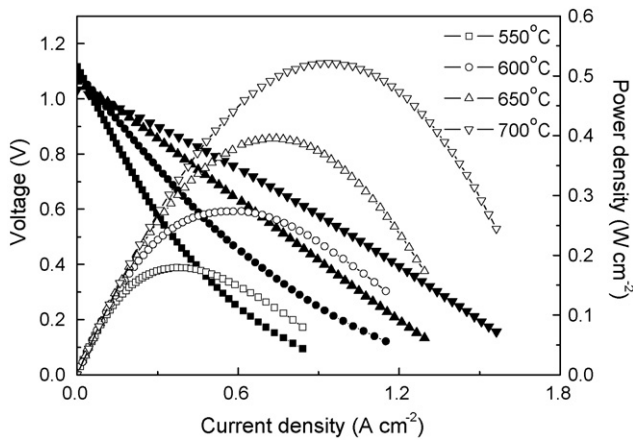
Fig. 4. Performance of the single cell under humidified hydrogen atmosphere at different temperatures.
